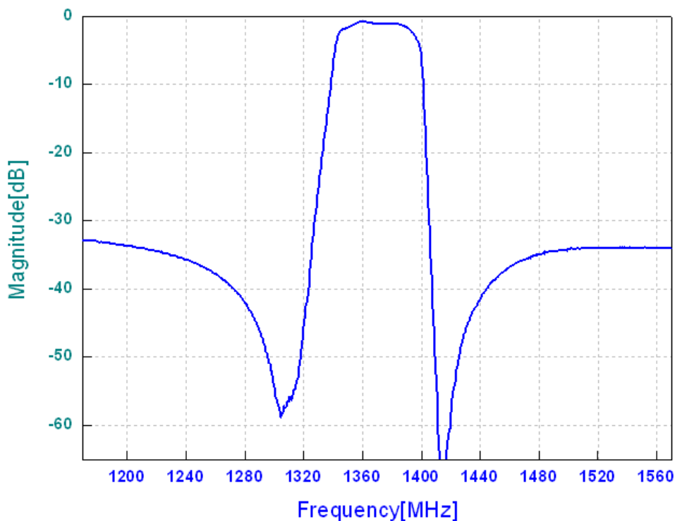
Frequency Response
